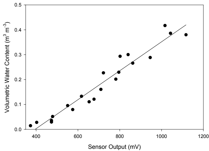
Fig. 2. Linear regression of soils with low to moderate sand content. Regression R^2 was 0.94.
