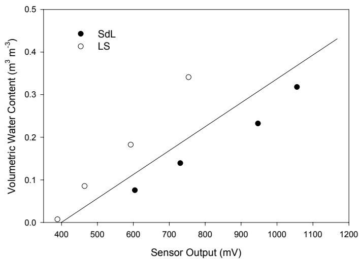
Fig. 3. Sensor output for soils with high sand content. Line indicates overall calibration line for soils with low to moderate sand content.
